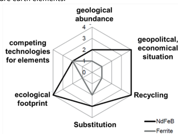
Fig. Spider chart (0 – no risk, 4 – high risk) analysing the criticality factors of metals – here a comparison of high performance NdFeB permanent magnet with low cost-low performance hard ferrite.
