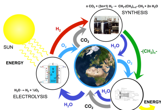
Fig. Schematic representation of the closed materials cycle, where hydrogen is produced from renewable energy and used together with \text{CO}_2 from the atmosphere to synthesize hydrocarbons as \text{CO}_2 neutral energy carriers.
